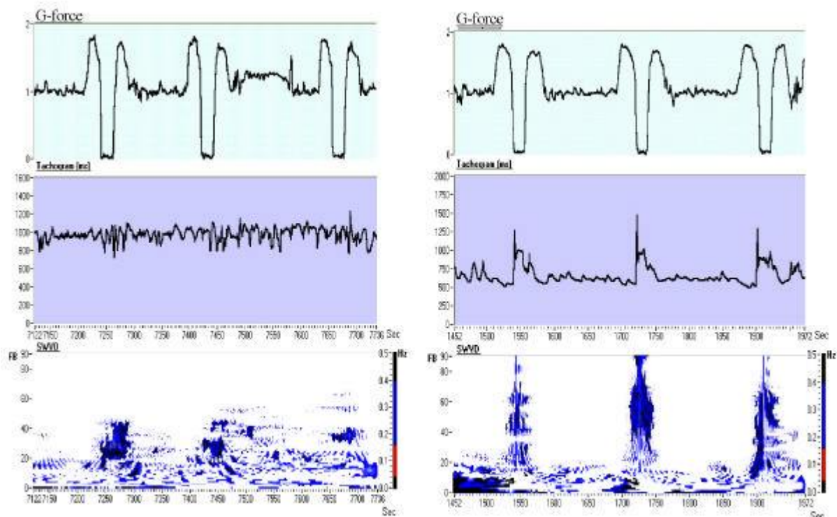
Fig 3. Left: supine subject, Right: standing subject. Upper: g force during 3 successive parabolas, Middle: tachogram, Lower: SWVD for same subject
